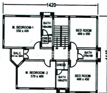
FIRST FLOOR PLAN BUILTUP AREA - 147.86 SQM
